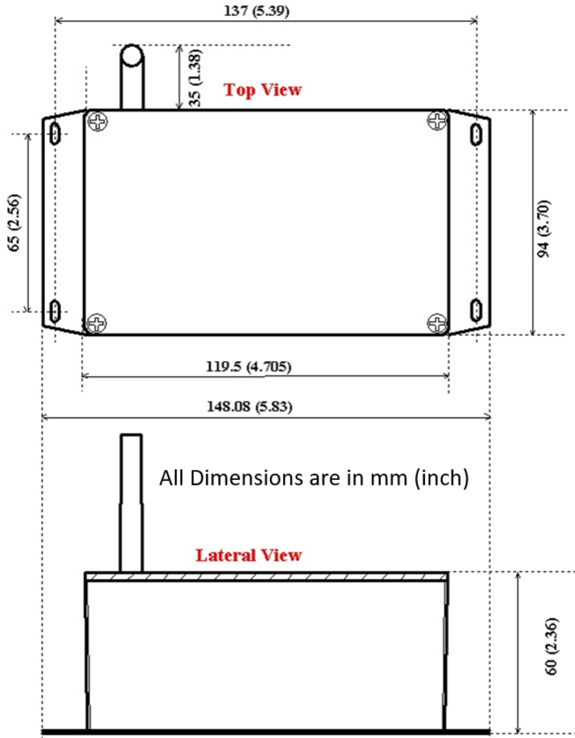
Figure 1: Wireless transceiver dimensions for wireless level meter. All measurements are in mm [inch].
